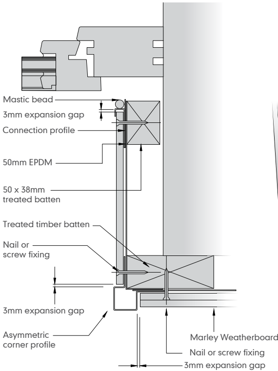
Detailing with asymmetric external corner trims at window jamb
